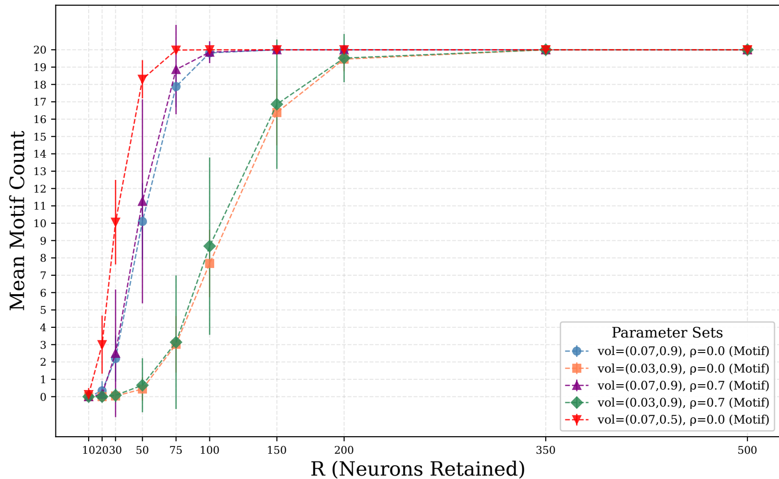
Mean Motif Counts vs Neuron Threshold (R) with R Thresholds for 50% Retention
